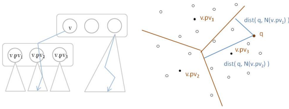
Figure 1: Metric Tree with k = 3 .
