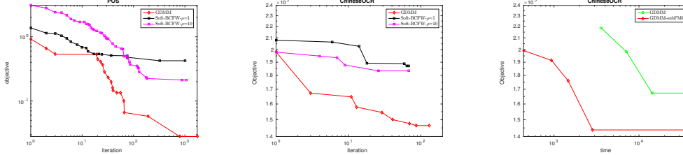
Figure 2: (left) Compare two FMO-based algorithms (GDMM, Soft-BCFW) in number of iterations. (right) Improvement in training time given by sublinear-time FMO.
